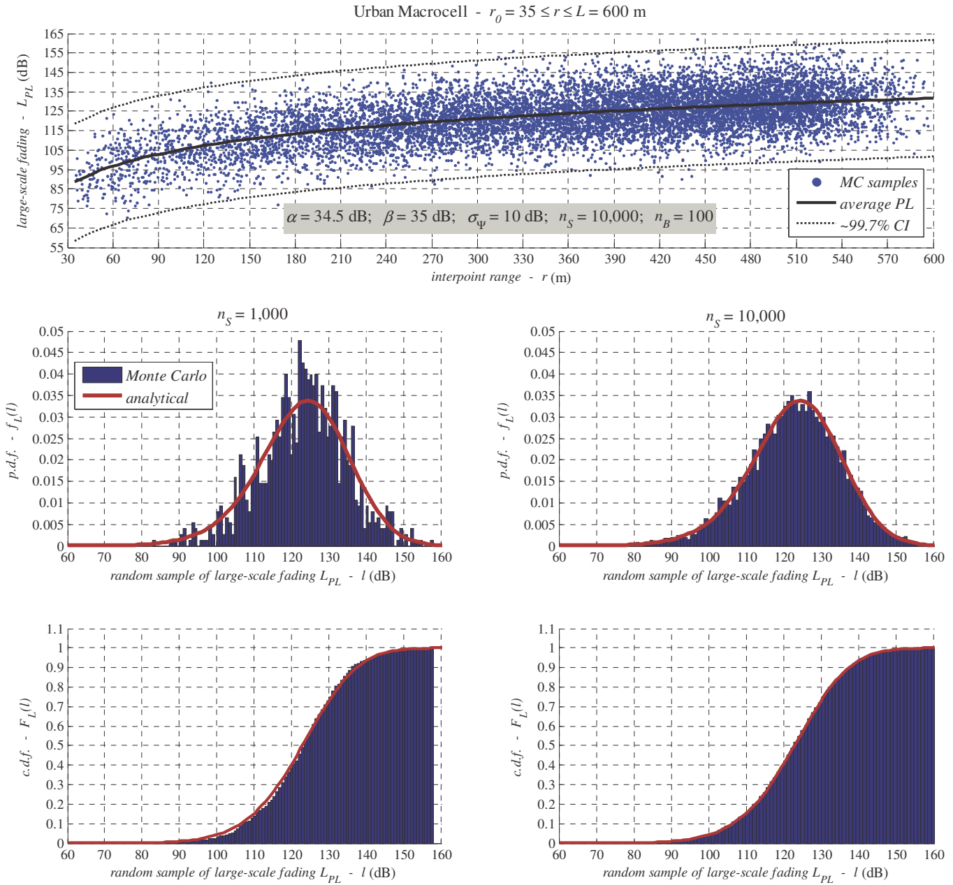
Figure 3.27 – Verifying the analytically derived formulation for large-scale fading PDF
