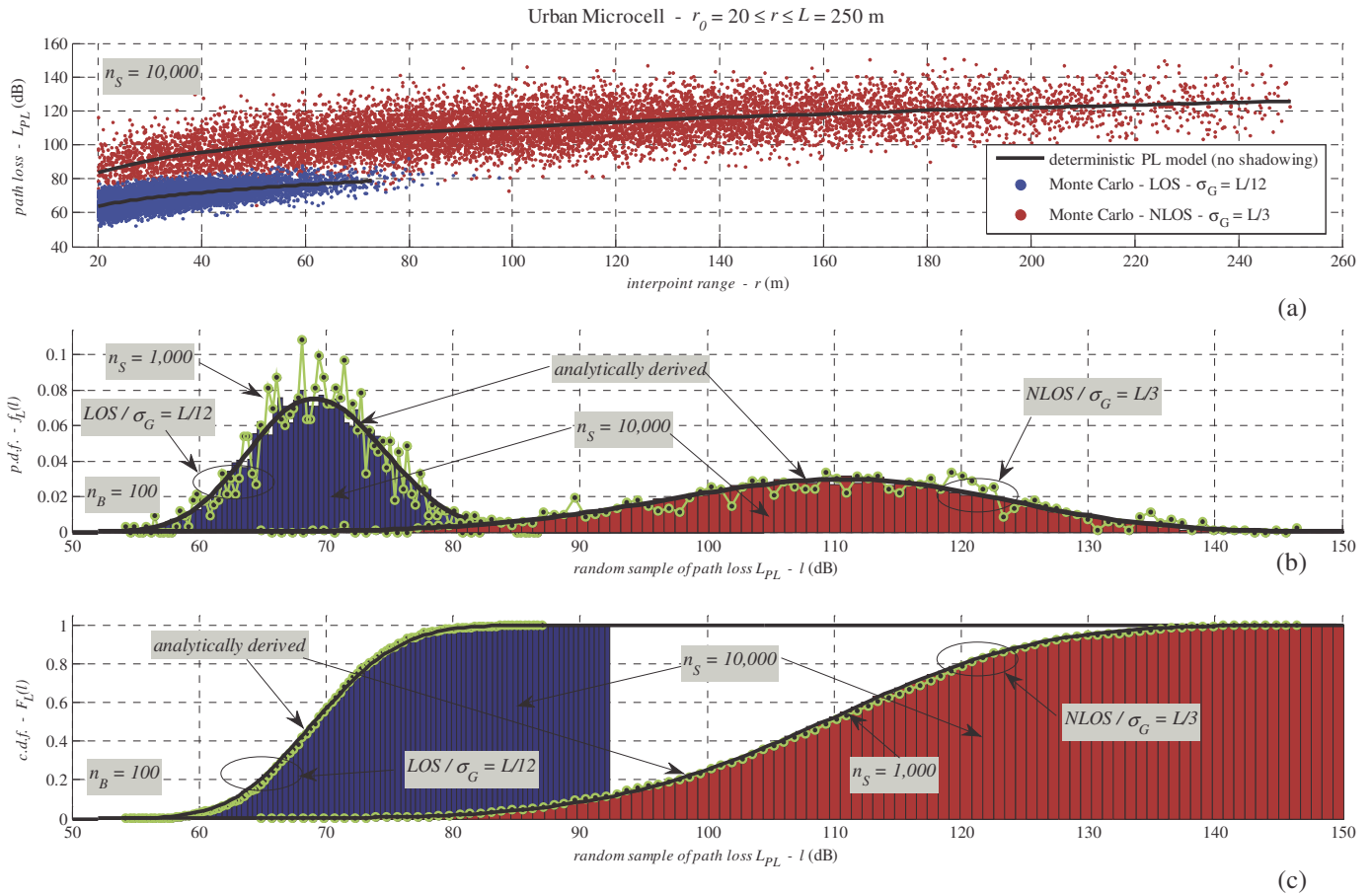
Figure 5.9 – Substantiating analytical derivation using the IEEE 802.20 channel
