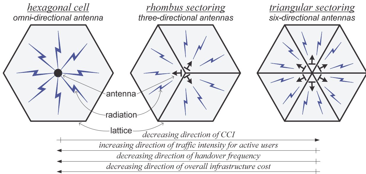
Figure 4.32 – Antenna radiation for unsectorized and sectorized cells
