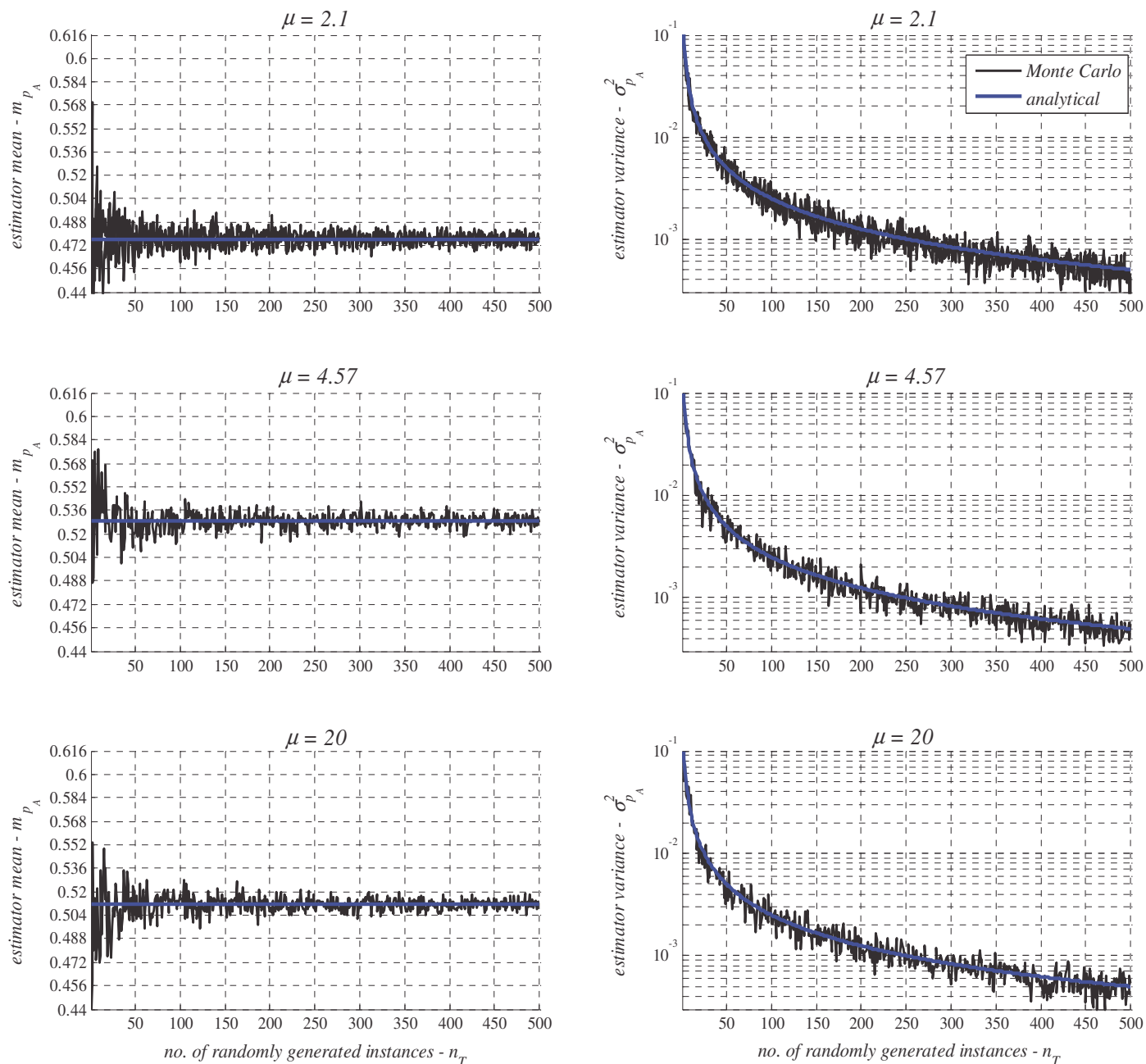
Figure 3.14 – Mean and variance of acceptance rate estimator over different RCR values
