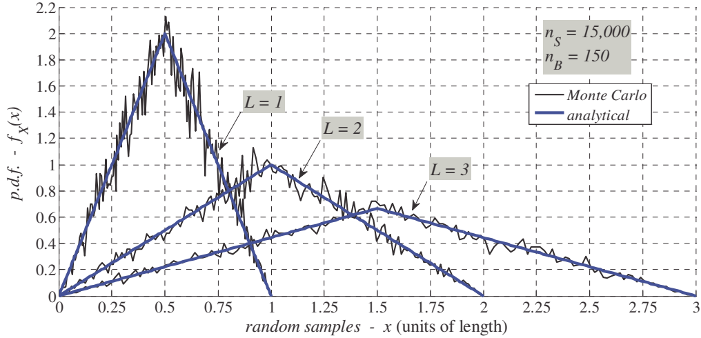
Figure 4.38 – Marginal PDF of nodal geometry for a triangular network along the x-axis
