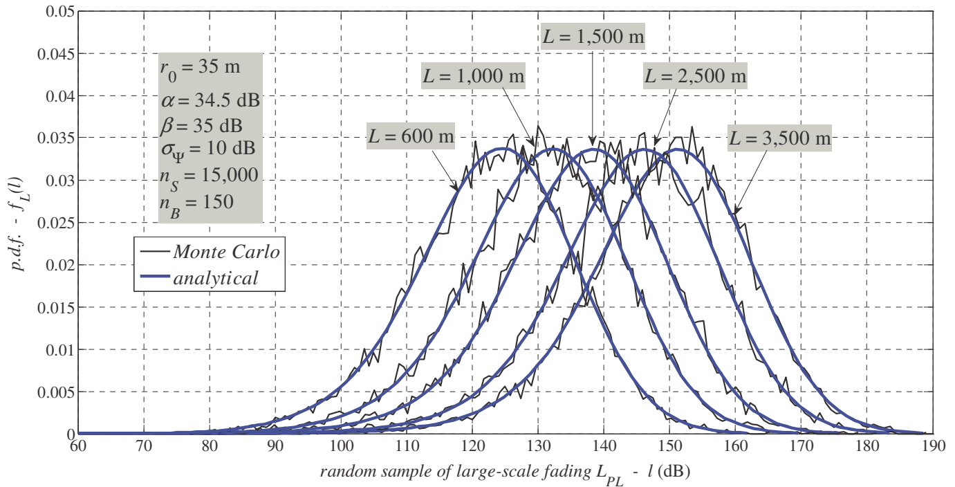
Figure 3.28 – Large-scale fading PDF for BS-to-MS over different cellular sizes
