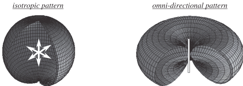
Figure 2.2 – All-direction antenna radiation models (3D) [49]
